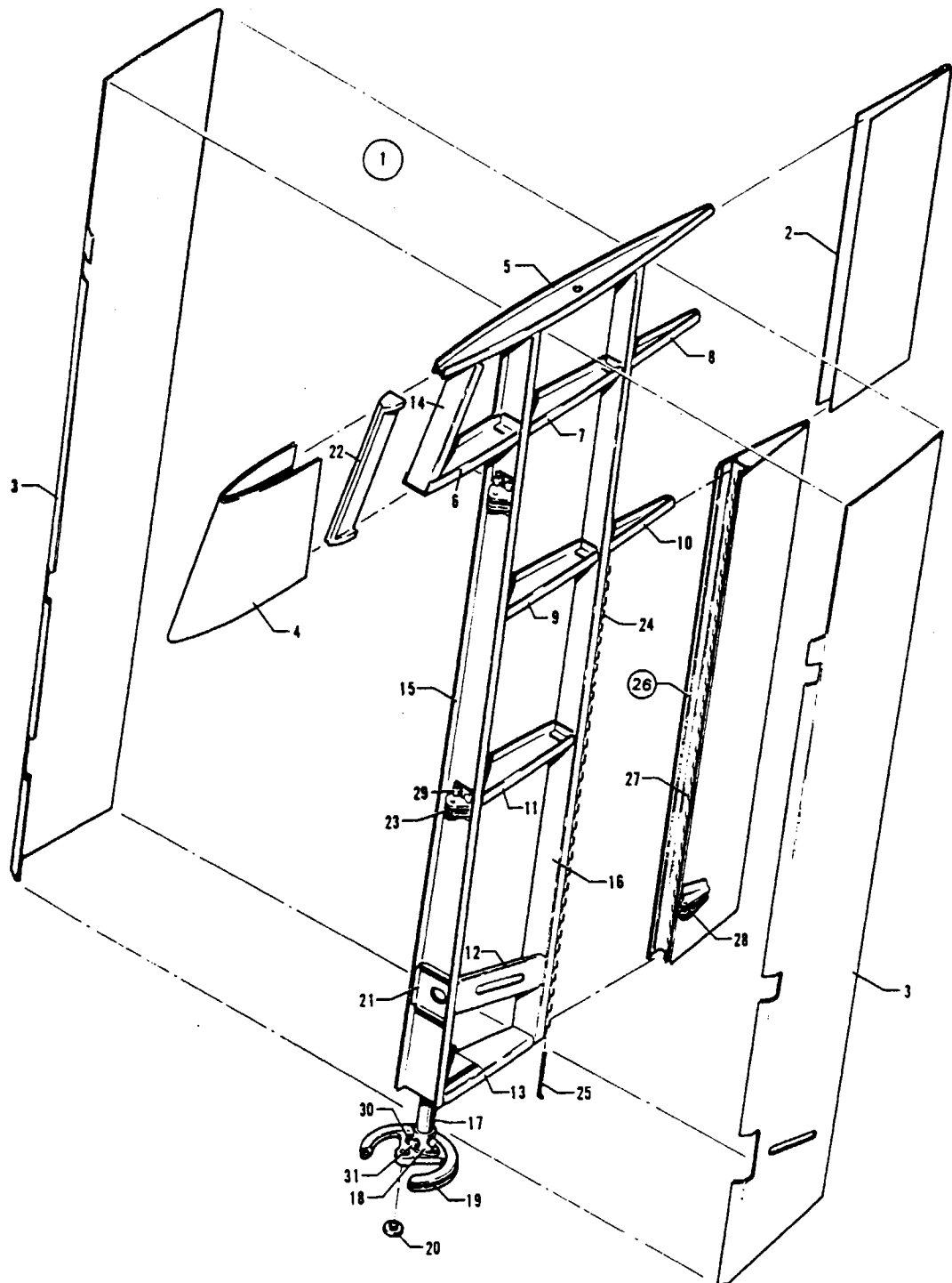
Figure 41 Rudder Assembly
