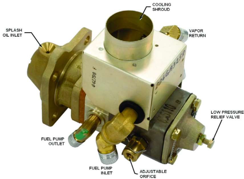
Typical Natural Aspirated Engine Driven Fuel Pump
