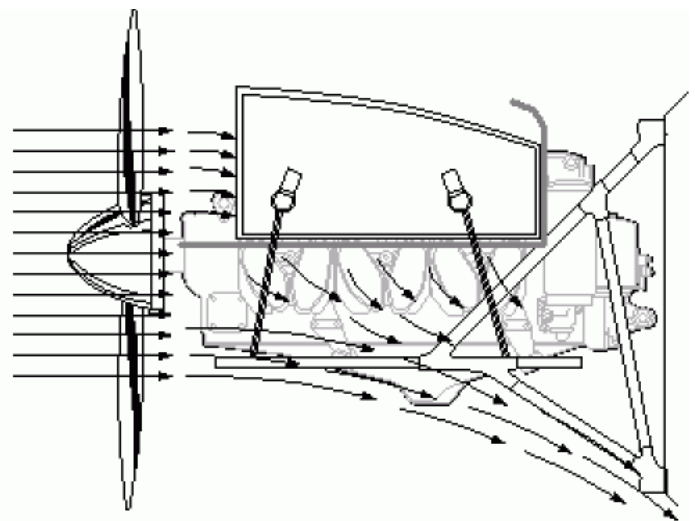
Figure 8. Sheet Metal Air Scoop Installed over Uncowled Engine.
