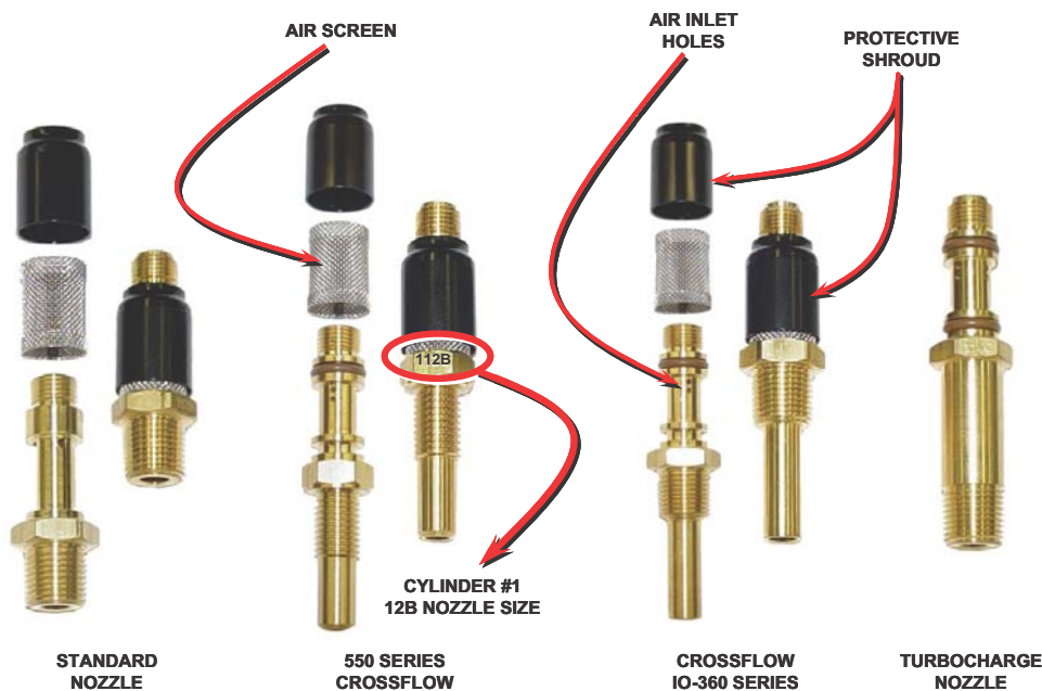
Position Tuned Fuel Injection Nozzles
